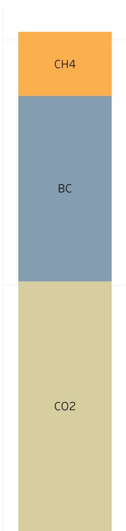
Off-road by pollutant
