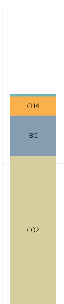
Marine by pollutant
