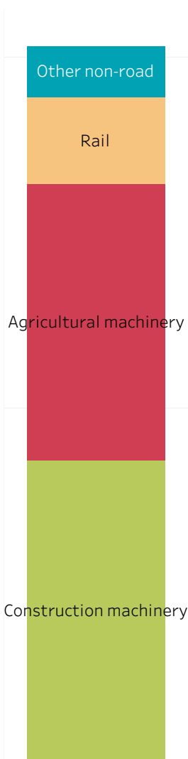
Off-road by sub-sector
