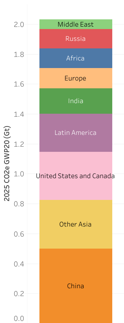
Off-road by region
